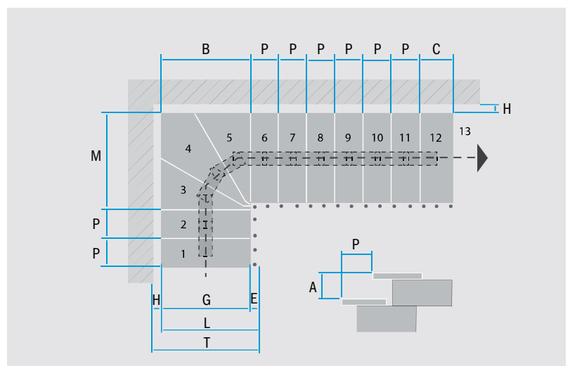
plan view with dimensions
