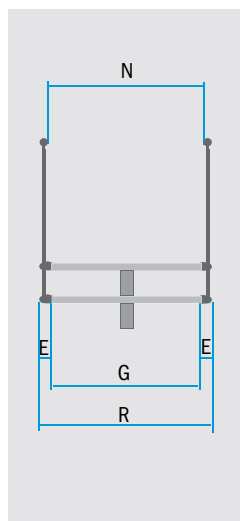
front view with railing on 2 sides
